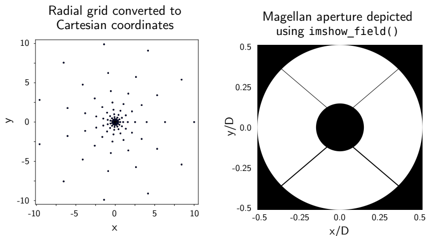
Figure 1: The resulting plots from the code in Listing 1. ( left ) The points for a separated grid using polar coordinates. ( right ) The Magellan aperture evaluated using supersampling on a pupil grid.
