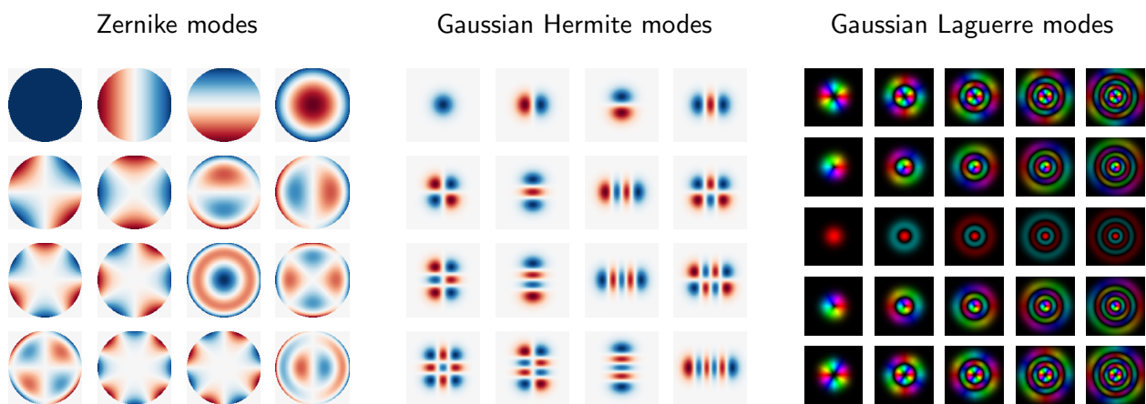
Figure 2: Some of the supported mode bases in HCIPy. This is the result of Listing 2.
