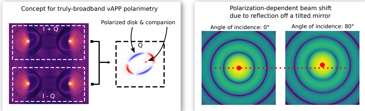
Figure 6: Some examples of polarization effects that can be simulated. (left) A truly-broadband vAPP implementation for polarimetry. A double difference detection scheme is simulated. This figure is adapted from Bos et al. 35 (right) The effect of polarization due to reflection off a tilted aluminum-coated mirror. This figure is courtesy of Rob van Holstein, work to appear in Van Holstein et al. in prep..
