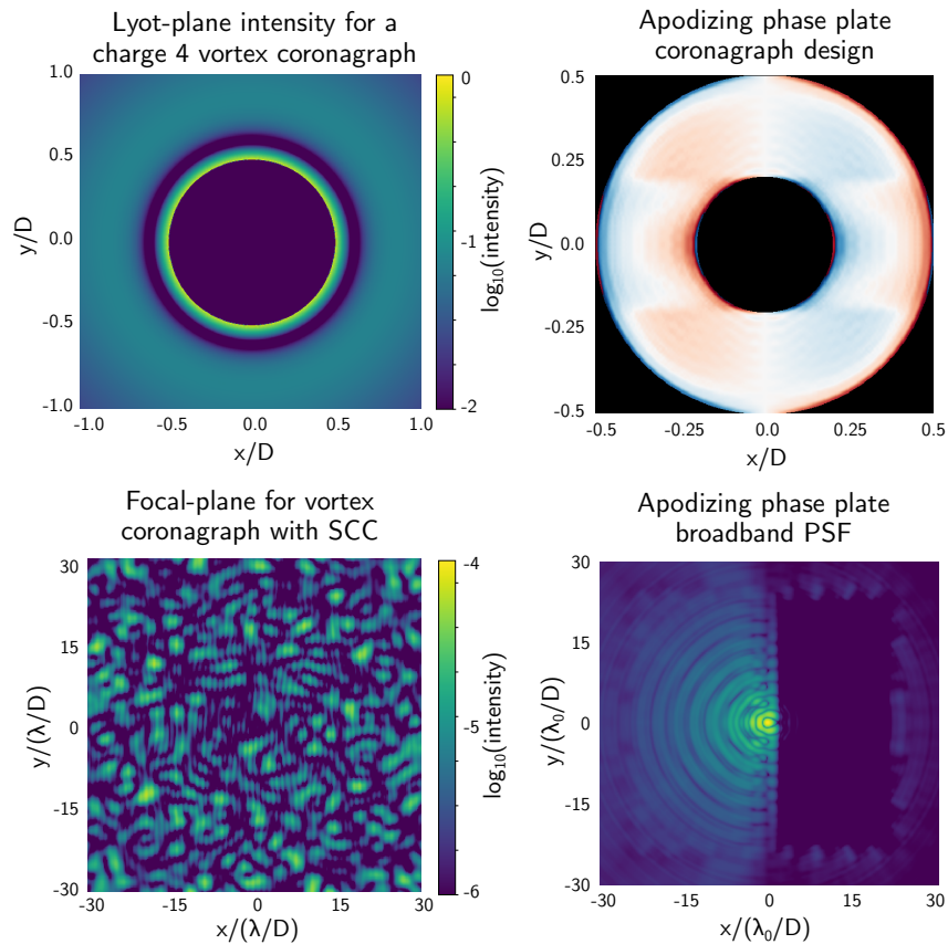
Figure 5: A series of simulated coronagraphic images with HCIPy. ( top left ) The Lyot-plane field for a charge 4 vortex coronagraph. ( bottom left ) The focal-plane image of the vortex coronagraph, with a self-coherent camera 34 Lyot-stop mask. The code for generating this image can be found in Listing 5. ( top right ) An example apodizing phase plate design optimized using HCIPy. ( bottom right ) The broadband point spread function for this APP design.
