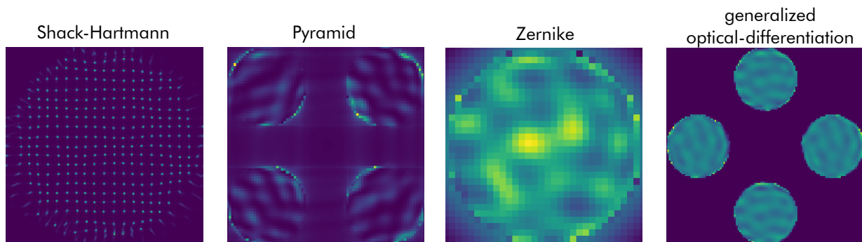
Figure 4: Simulated images for different wavefront sensors using HCIPy. All wavefront sensors see the same phase aberration. The amplitude of the aberration was scaled to approximately the linear range of the wavefront sensor, for visualization purposes.
