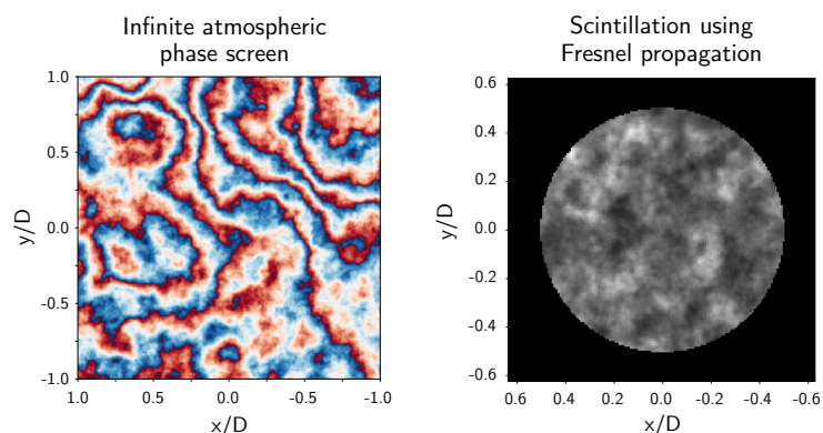
Figure 3: The simulated images from Listing 3. These images show a simulated phase screen that can be extruded infinitely in any direction ( left ), and the scintillation from a series of phase screens with Fresnel propagation between layers ( right ).
